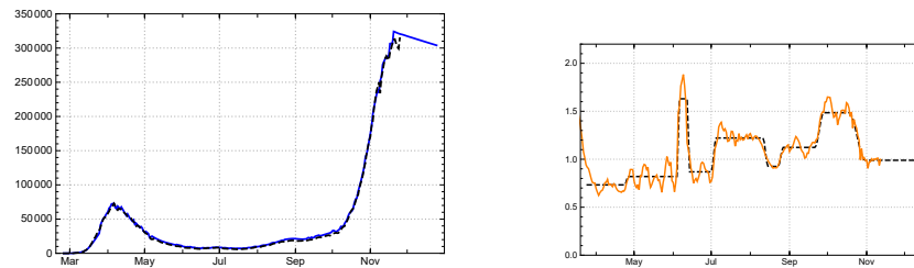
FIGURE 2. Left: SEPIR model for the number of actual infections I based on data until Nov 25, 2020; JHU data black dashed, model values blue. Right: SEPIR reproduction numbers (orange) on the basis of JHU data for daily new infected, model values with constancy intervals black dashed.
